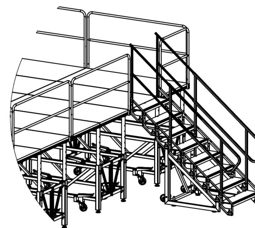
DETAIL A SCALE 1 : 40
